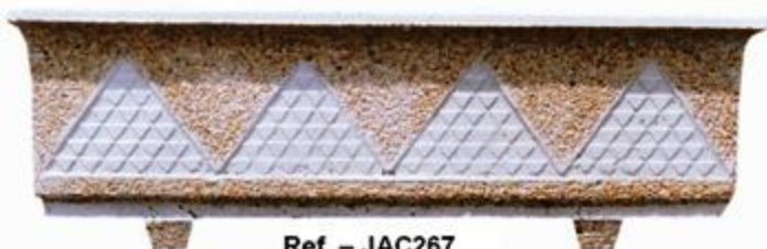
Ref. - JAC267 Haut. 30 cm Long. 80 cm Larg. 25 cm Poids 27 kg
